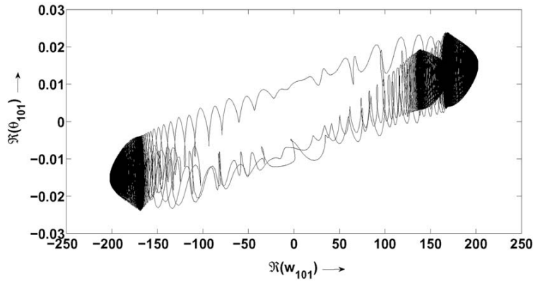
Figure 3. Projection of the phase space in the \Re(W_{101}) - \Re(\theta_{101}) plane at r = 830 . The figure illustrates the chaotic behaviour of the system.
