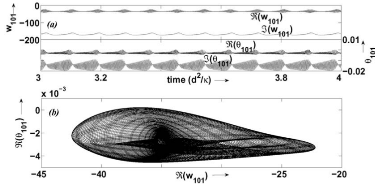
Figure 1. (a) Time series of \Re(W_{101}) , \Im(W_{101}) , \Re(\theta_{101}) , \Im(\theta_{101}) at reduced Rayleigh number r = 700 and Prandtl number P = 6.8 . The time series has two leading frequencies, and it shows quasiperiodic behaviour. (b) The projection of the phase space in \Re(W_{101}) - \Re(\theta_{101}) that elucidates the quasiperiodic behaviour of the system.
