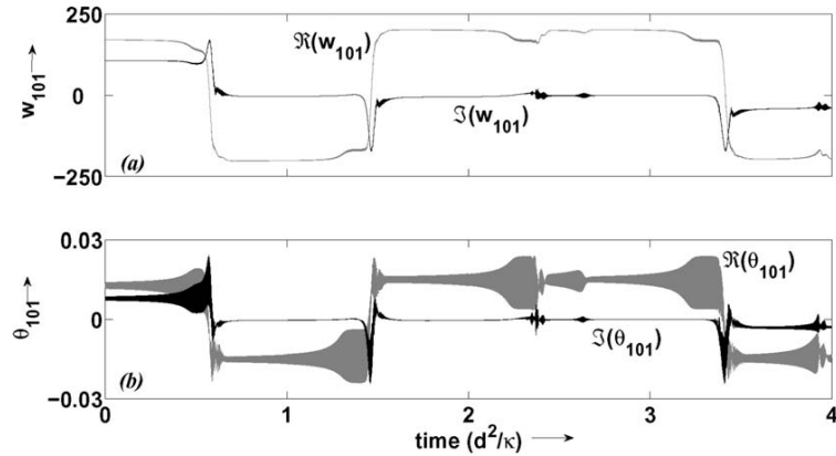
Figure 2. Time series of the real and imaginary parts of the critical velocity mode W_{101} (a) and the temperature mode \theta_{101} (b) for r = 830 . The origin on dimensionless time axis is suitably chosen after the steady state has been reached. The time series of the modes shows jitters (small fluctuations) and flips. The fluctuations in the temperature mode is stronger than that in the velocity mode.
