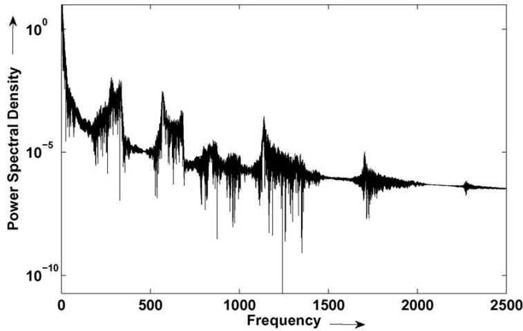
Figure 4. Power spectral density plot for the time signal of \Re(W_{101}) obtained from DNS of 2D RBC at r = 830 and P = 6.8 .
