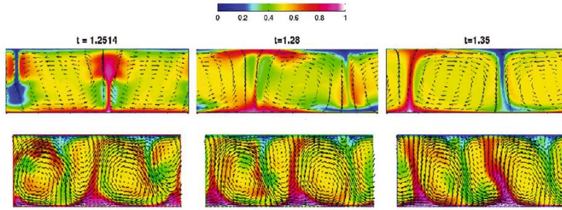
Figure 5. Travelling rolls in two-dimensional Rayleigh–Bénard convection at r = 830 . The top panel of the figures is for the simulation with free-slip boundaries and the bottom panel is for the no-slip boundaries. The temperature field is represented in colour with blue being the coldest region. The arrows represent the velocity field. The three images at the top panel show the field configurations at three time. At t = 1.2514 the central region has hot fluid that shifts leftward subsequently. At t = 1.35 the whole roll pattern is shifted approximately by half a wavelength. Similar features are seen for no-slip convective flow, except that the flow pattern moves right.
